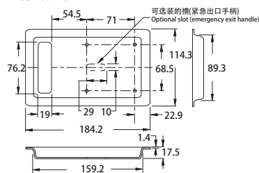
U型支架 U-shaped bracket (包含用于紧急出口手柄的槽) (Contains slots for emergency exit handles)
