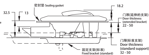
后视图Rear View
