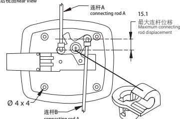
后视图Rear View
