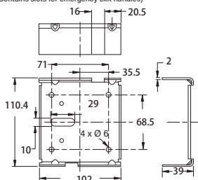
U型支架 U-shaped bracket (包含用于紧急出口手柄的槽) (Contains slots for emergency exit handles)
