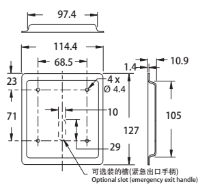
延伸的支架Extended bracket
