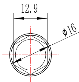
M8型号螺栓 M8 model bolt
