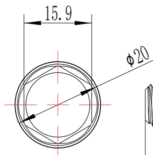
M10型号螺栓 M10 model bolt
