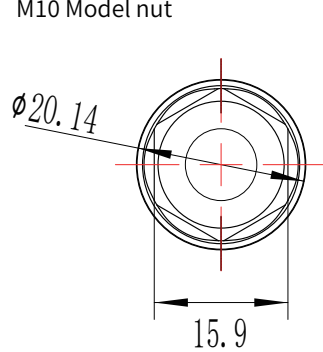
M10型号螺帽 M10 Model nut
